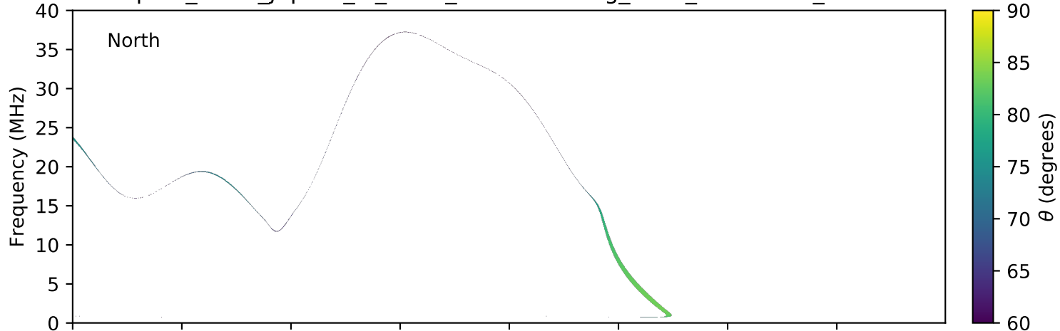
expres_earth_jupiter_io_isaac_lossc-wid1deg_3kev_20070207_v01.cdf
