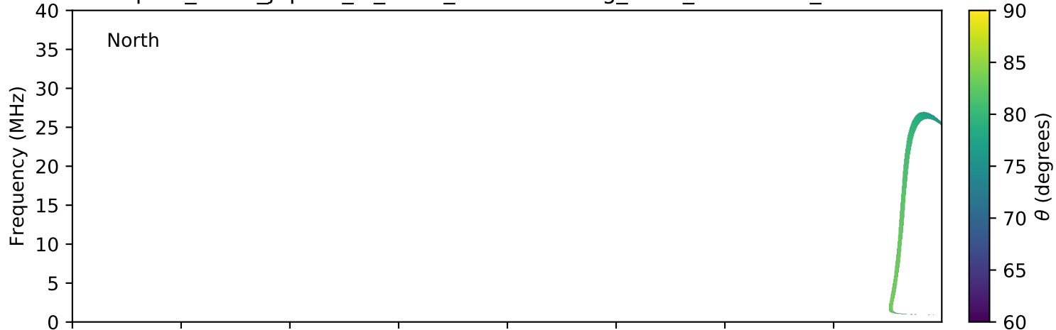
expres_earth_jupiter_io_isaac_lossc-wid1deg_3kev_20070206_v01.cdf
