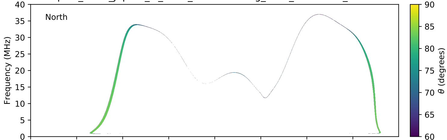
expres_earth_jupiter_io_isaac_lossc-wid1deg_3kev_20070205_v01.cdf
