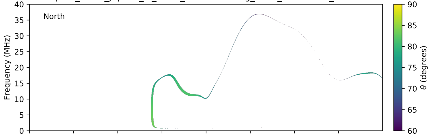
expres_earth_jupiter_io_isaac_lossc-wid1deg_3kev_20070203_v01.cdf
