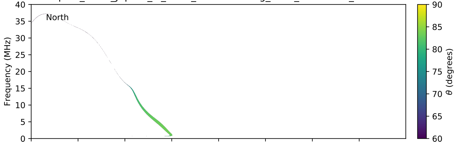
expres_earth_jupiter_io_isaac_lossc-wid1deg_3kev_20070202_v01.cdf
