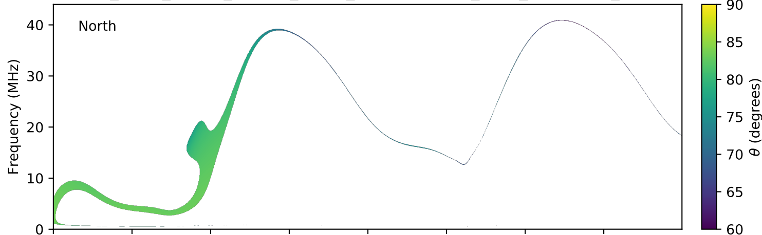
expres_earth_jupiter_europa_jrm09_lossc-wid1deg_3kev_20070225_v01.cdf
