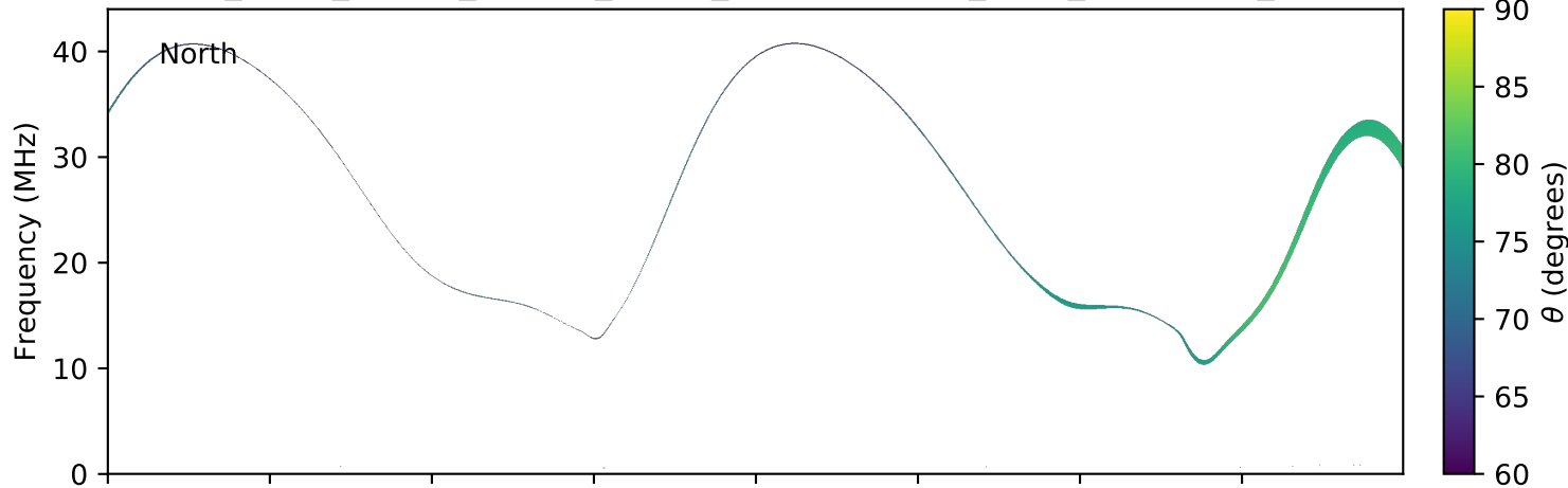
expres_earth_jupiter_europa_jrm09_lossc-wid1deg_3kev_20070222_v01.cdf
