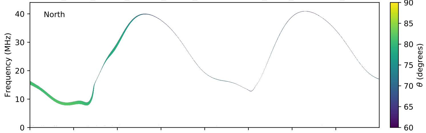
expres_earth_jupiter_europa_jrm09_lossc-wid1deg_3kev_20070218_v01.cdf
