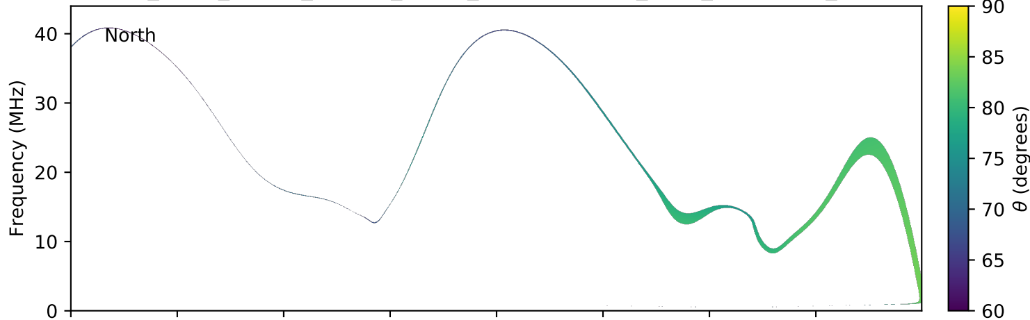
expres_earth_jupiter_europa_jrm09_lossc-wid1deg_3kev_20070215_v01.cdf
