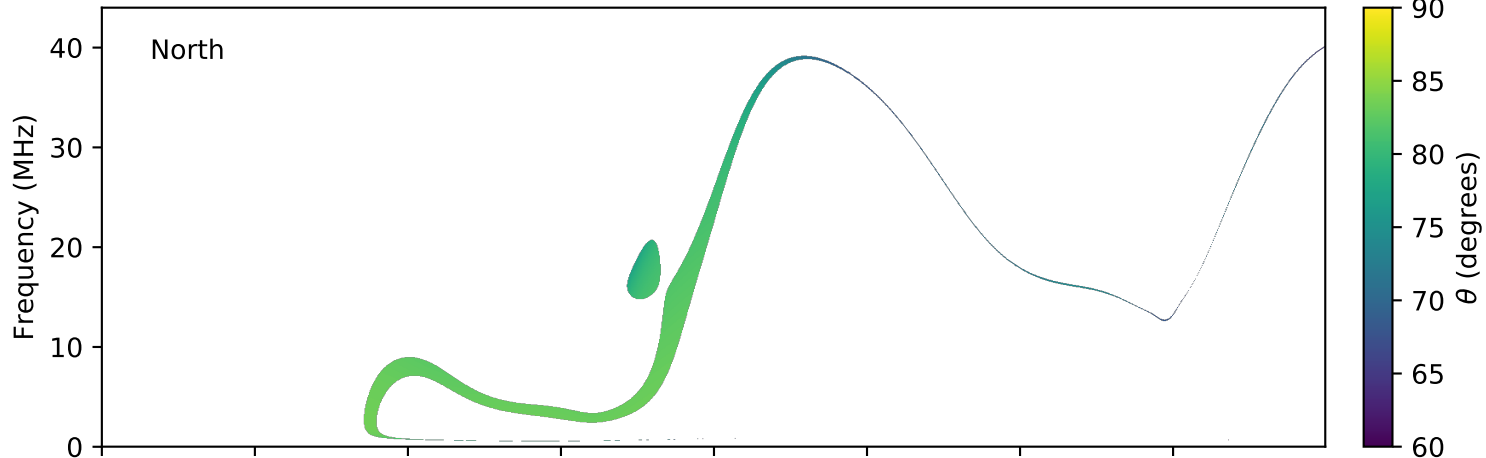
expres_earth_jupiter_europa_jrm09_lossc-wid1deg_3kev_20070207_v01.cdf
