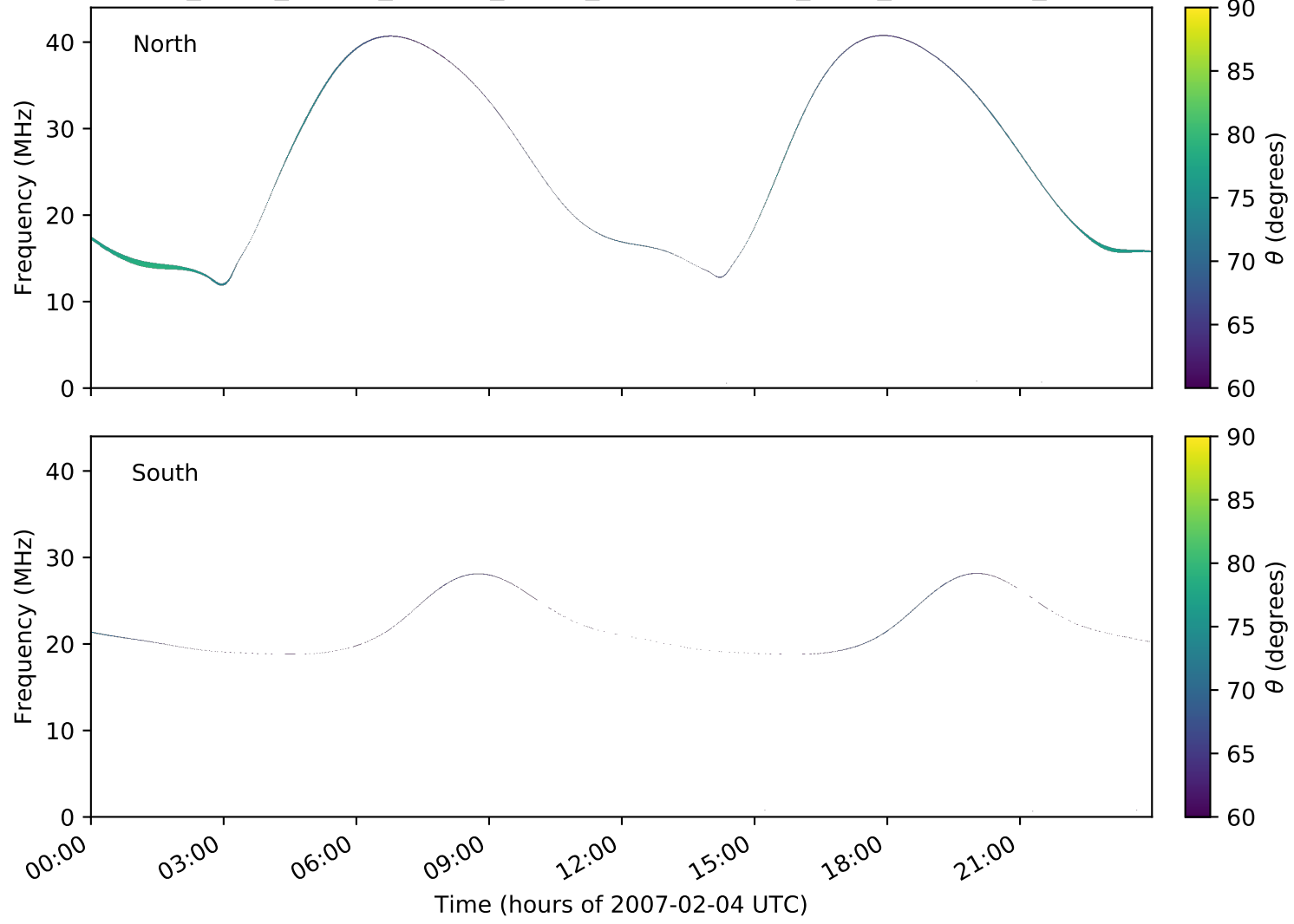
expres_earth_jupiter_europa_jrm09_lossc-wid1deg_3kev_20070204_v01.cdf
