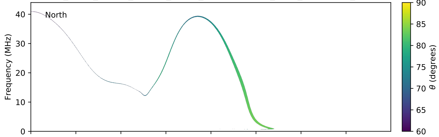
expres_earth_jupiter_europa_jrm09_lossc-wid1deg_3kev_20070201_v01.cdf
