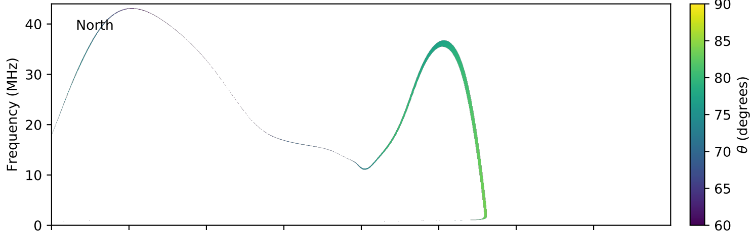
expres_earth_jupiter_io_jrm09_lossc-wid1deg_3kev_20070131_v01.cdf
