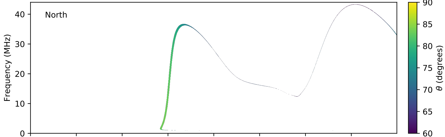
expres_earth_jupiter_io_jrm09_lossc-wid1deg_3kev_20070127_v01.cdf
