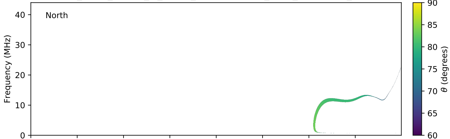
expres_earth_jupiter_io_jrm09_lossc-wid1deg_3kev_20070123_v01.cdf
