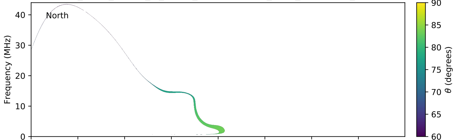
expres_earth_jupiter_io_jrm09_lossc-wid1deg_3kev_20070117_v01.cdf
