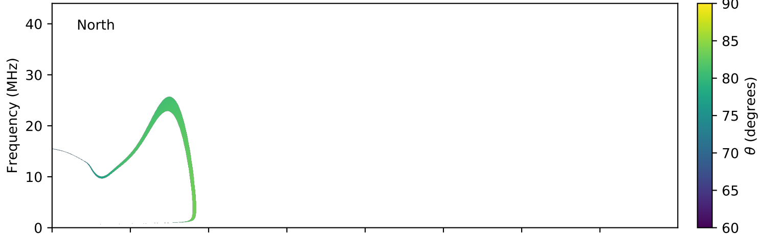
expres_earth_jupiter_io_jrm09_lossc-wid1deg_3kev_20070112_v01.cdf
