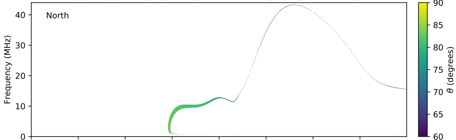
expres_earth_jupiter_io_jrm09_lossc-wid1deg_3kev_20070111_v01.cdf
