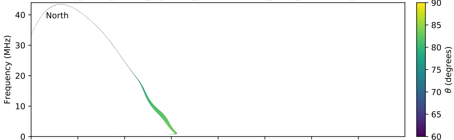
expres_earth_jupiter_io_jrm09_lossc-wid1deg_3kev_20070110_v01.cdf
