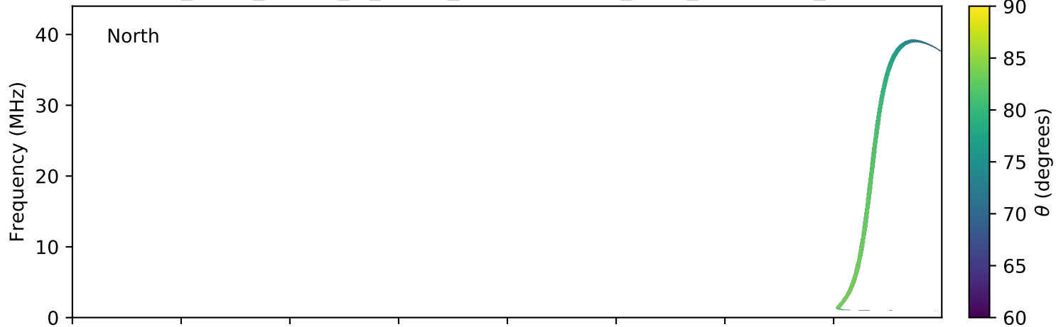
expres_earth_jupiter_io_jrm09_lossc-wid1deg_3kev_20070107_v01.cdf
