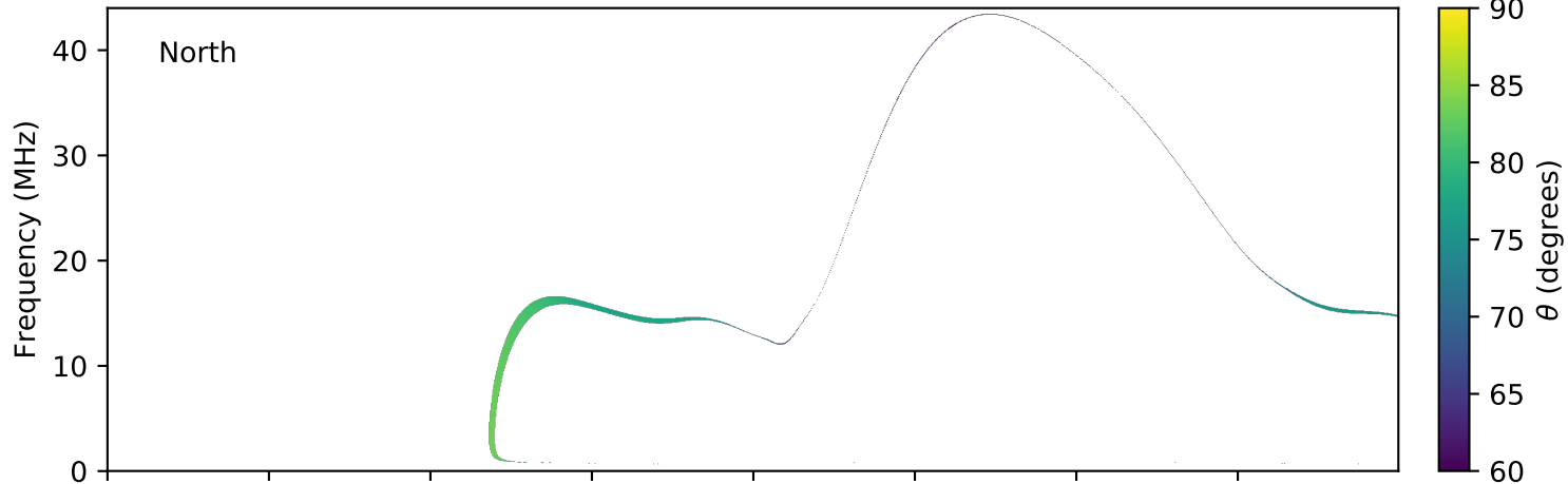
expres_earth_jupiter_io_jrm09_lossc-wid1deg_3kev_20070104_v01.cdf
