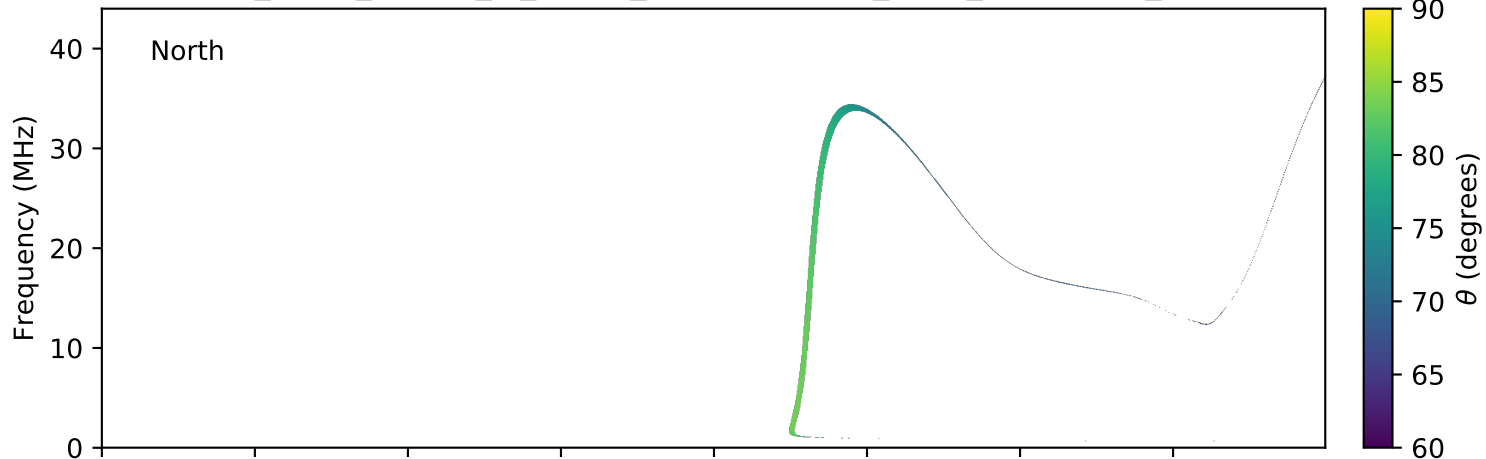
expres_earth_jupiter_io_jrm09_lossc-wid1deg_3kev_20070102_v01.cdf
