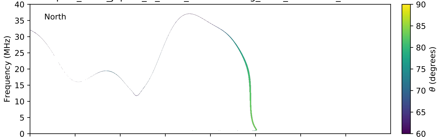
expres_earth_jupiter_io_isaac_lossc-wid1deg_3kev_20070131_v01.cdf
