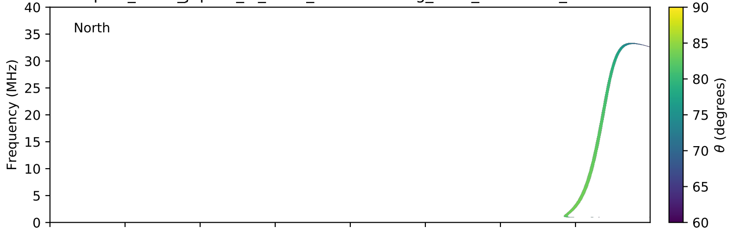
expres_earth_jupiter_io_isaac_lossc-wid1deg_3kev_20070130_v01.cdf
