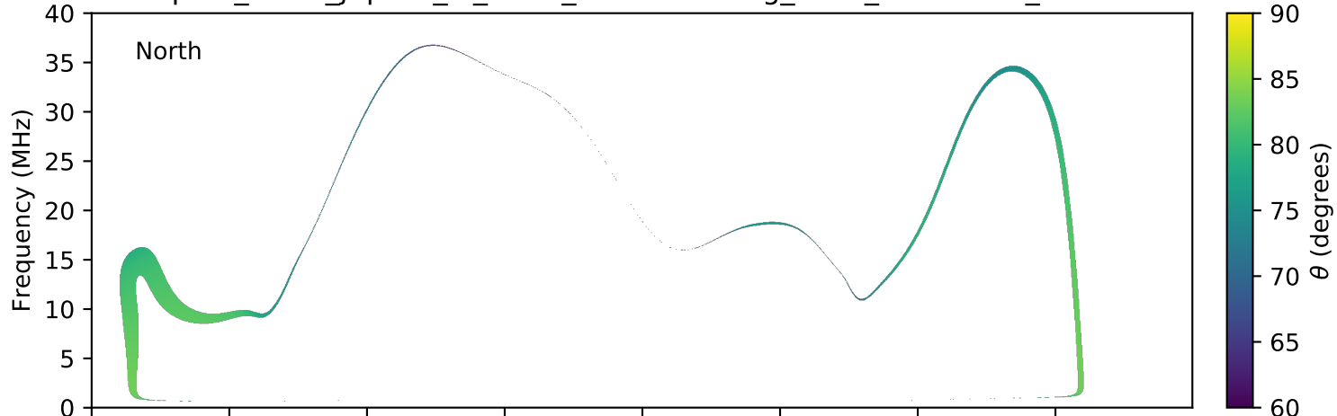
expres_earth_jupiter_io_isaac_lossc-wid1deg_3kev_20070129_v01.cdf
