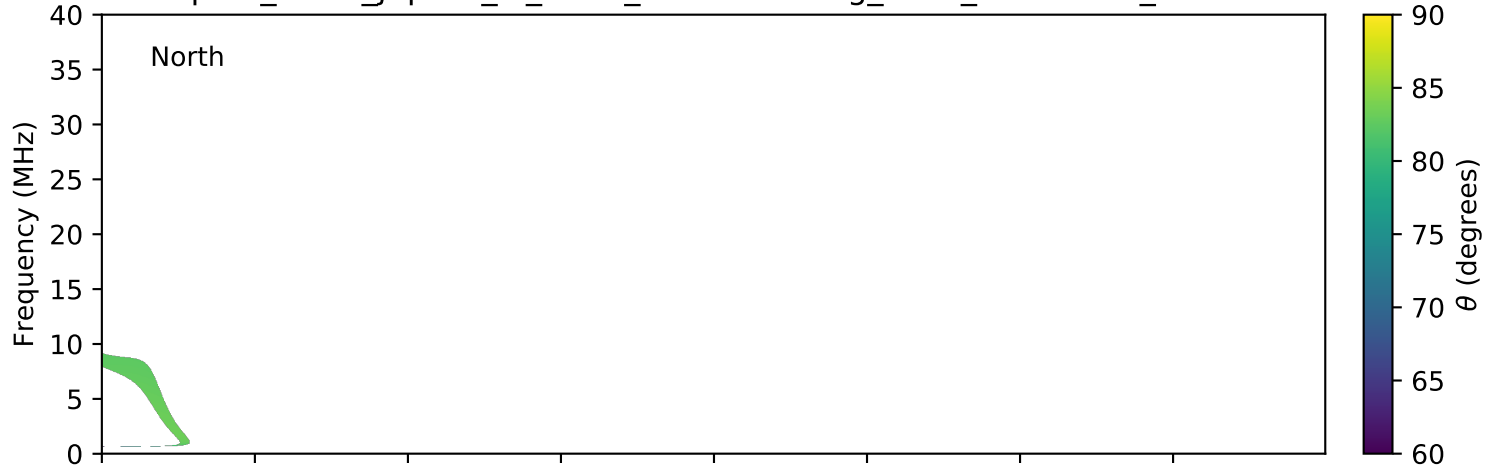
expres_earth_jupiter_io_isaac_lossc-wid1deg_3kev_20070128_v01.cdf
