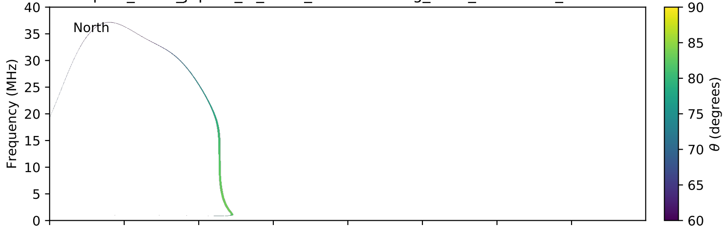
expres_earth_jupiter_io_isaac_lossc-wid1deg_3kev_20070126_v01.cdf
