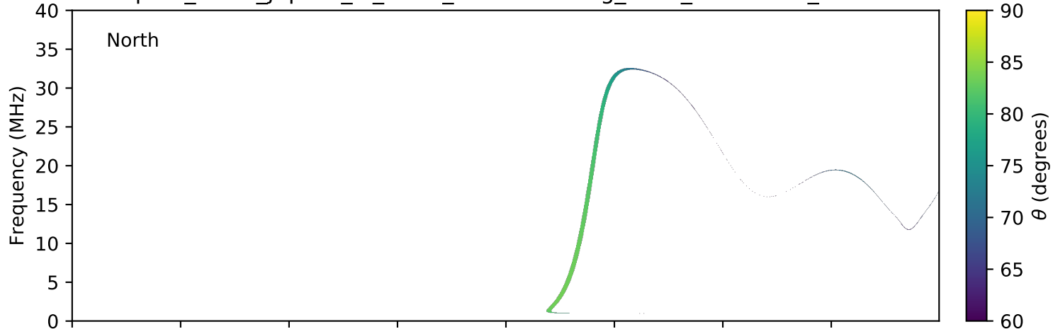
expres_earth_jupiter_io_isaac_lossc-wid1deg_3kev_20070125_v01.cdf
