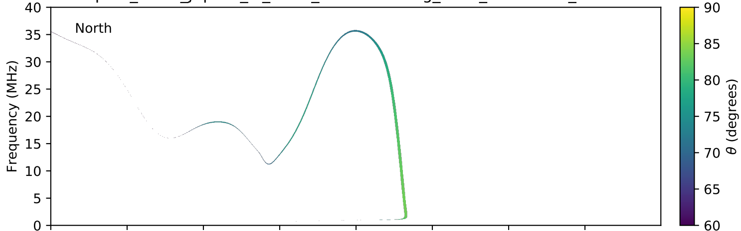
expres_earth_jupiter_io_isaac_lossc-wid1deg_3kev_20070124_v01.cdf
