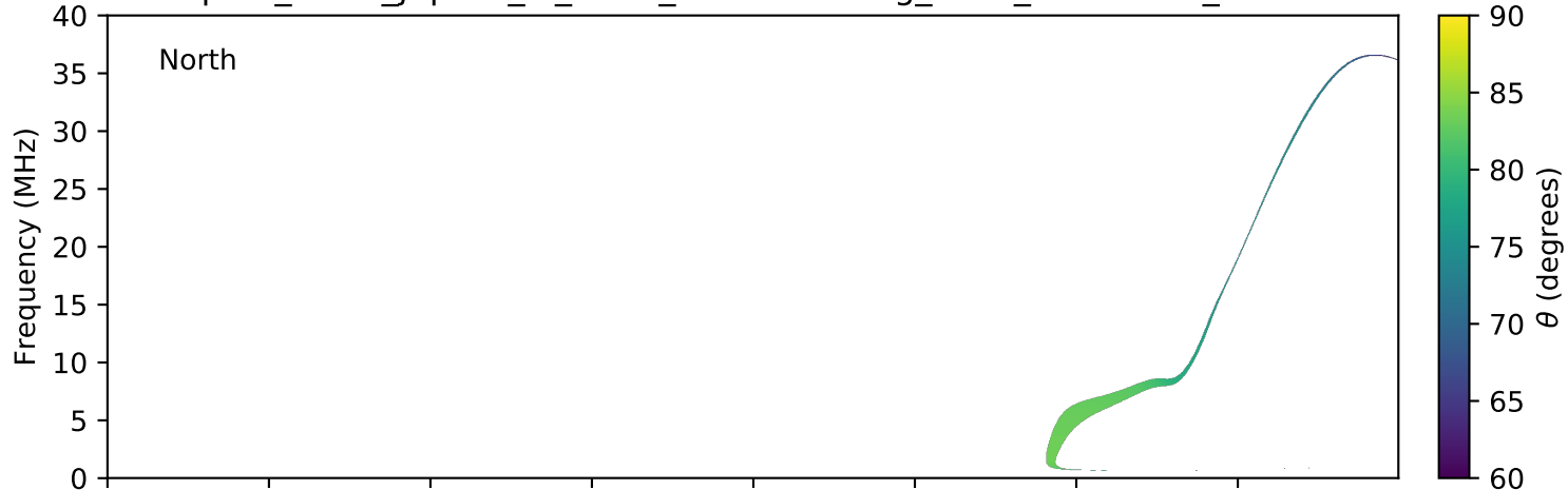
expres_earth_jupiter_io_isaac_lossc-wid1deg_3kev_20070123_v01.cdf
