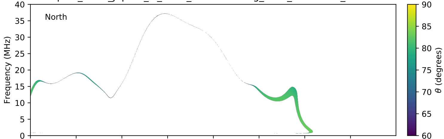
expres_earth_jupiter_io_isaac_lossc-wid1deg_3kev_20070122_v01.cdf
