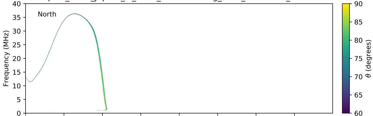
expres_earth_jupiter_io_isaac_lossc-wid1deg_3kev_20070119_v01.cdf
