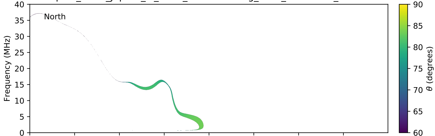
expres_earth_jupiter_io_isaac_lossc-wid1deg_3kev_20070117_v01.cdf
