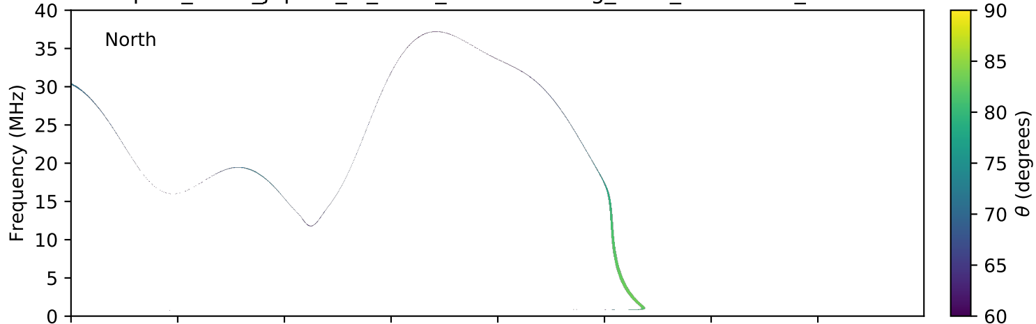
expres_earth_jupiter_io_isaac_lossc-wid1deg_3kev_20070115_v01.cdf
