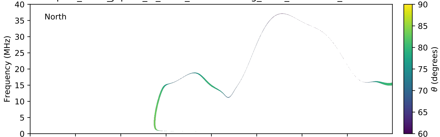
expres_earth_jupiter_io_isaac_lossc-wid1deg_3kev_20070111_v01.cdf
