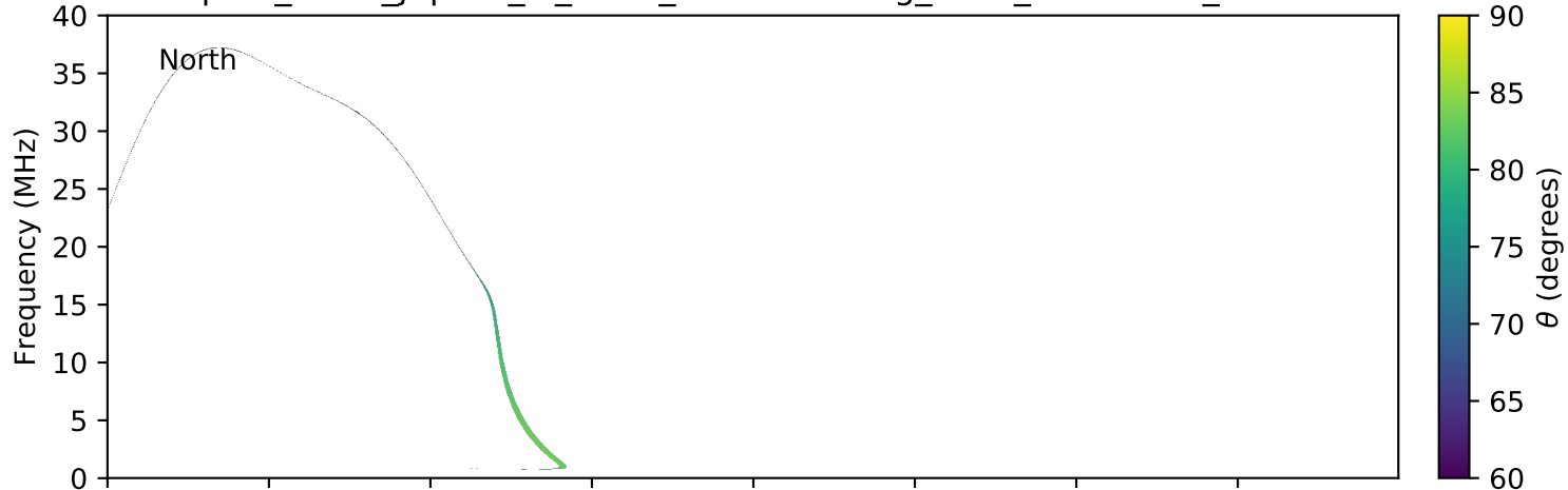
expres_earth_jupiter_io_isaac_lossc-wid1deg_3kev_20070110_v01.cdf
