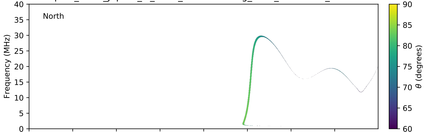
expres_earth_jupiter_io_isaac_lossc-wid1deg_3kev_20070109_v01.cdf
