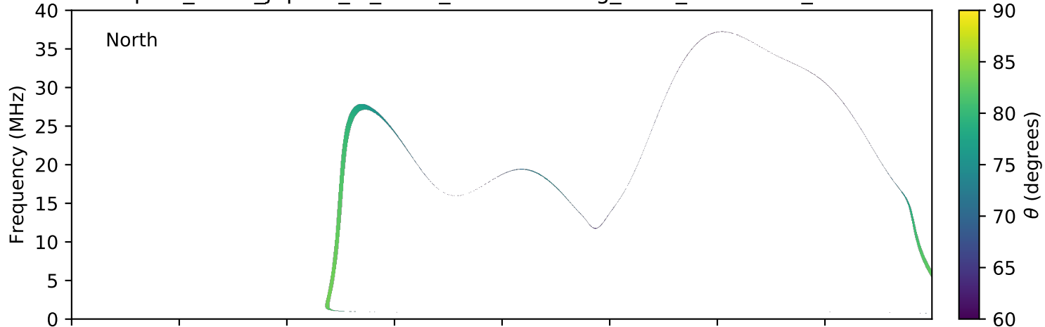
expres_earth_jupiter_io_isaac_lossc-wid1deg_3kev_20070104_v01.cdf
