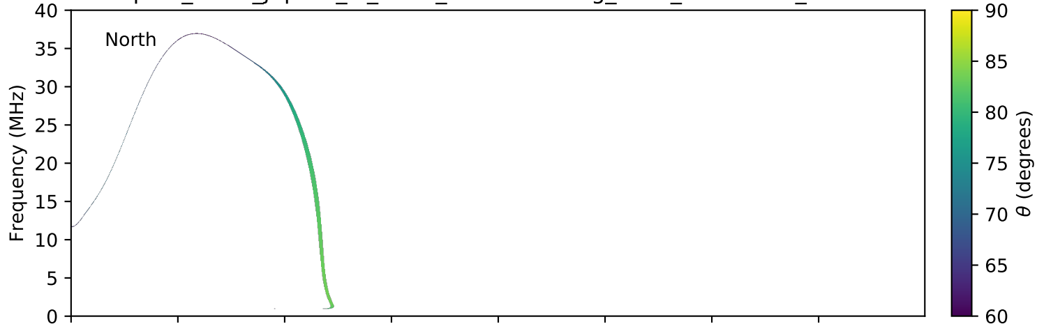
expres_earth_jupiter_io_isaac_lossc-wid1deg_3kev_20070103_v01.cdf
