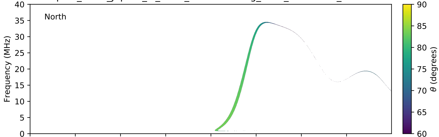
expres_earth_jupiter_io_isaac_lossc-wid1deg_3kev_20070102_v01.cdf
