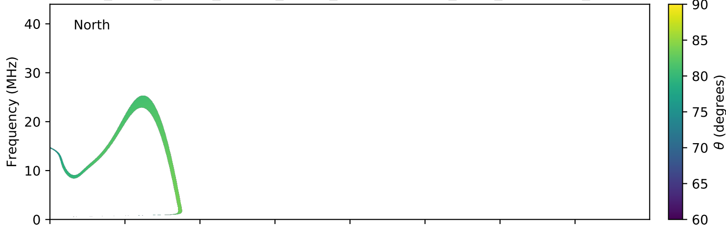
expres_earth_jupiter_europa_jrm09_lossc-wid1deg_3kev_20070129_v01.cdf
