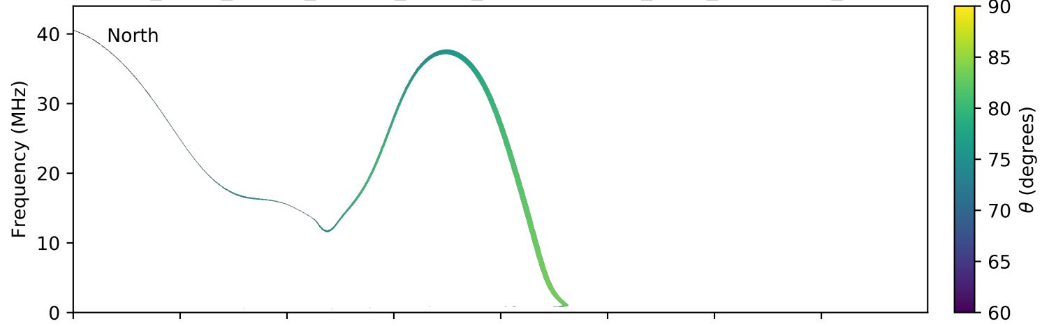
expres_earth_jupiter_europa_jrm09_lossc-wid1deg_3kev_20070125_v01.cdf
