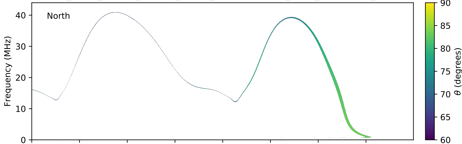
expres_earth_jupiter_europa_jrm09_lossc-wid1deg_3kev_20070114_v01.cdf
