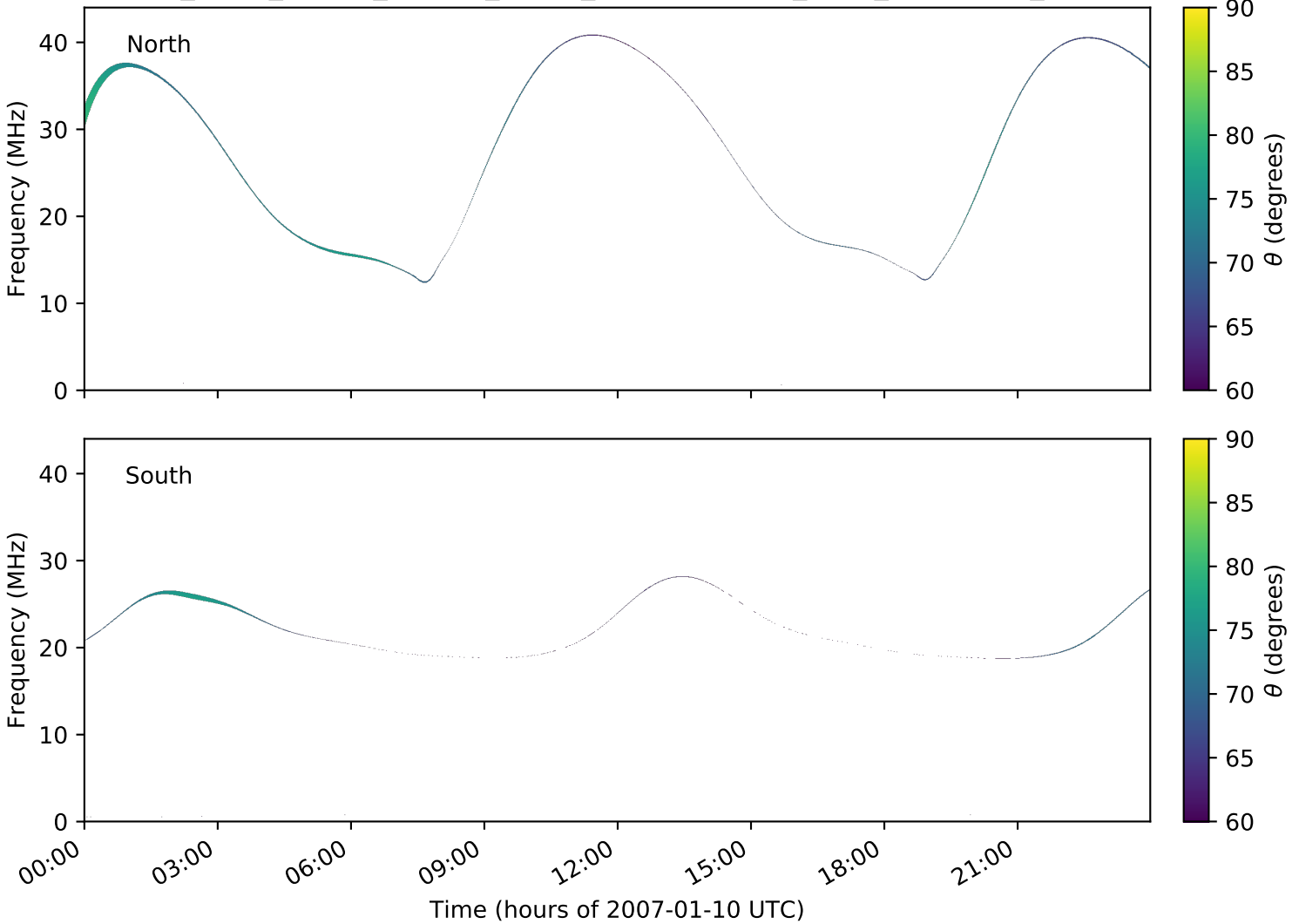
expres_earth_jupiter_europa_jrm09_lossc-wid1deg_3kev_20070110_v01.cdf
