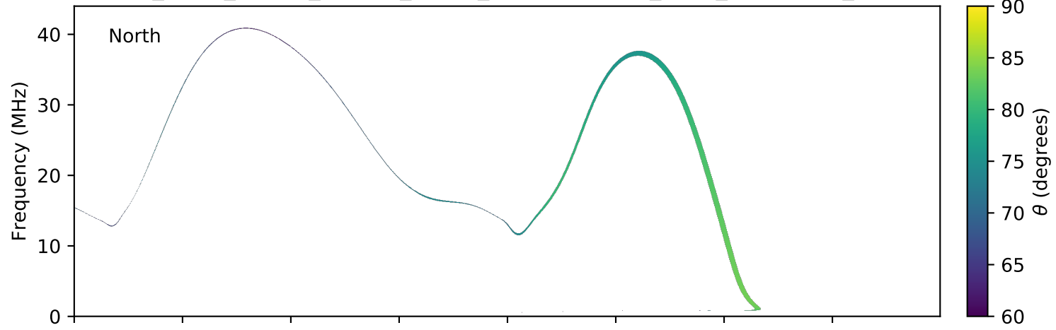
expres_earth_jupiter_europa_jrm09_lossc-wid1deg_3kev_20070107_v01.cdf
