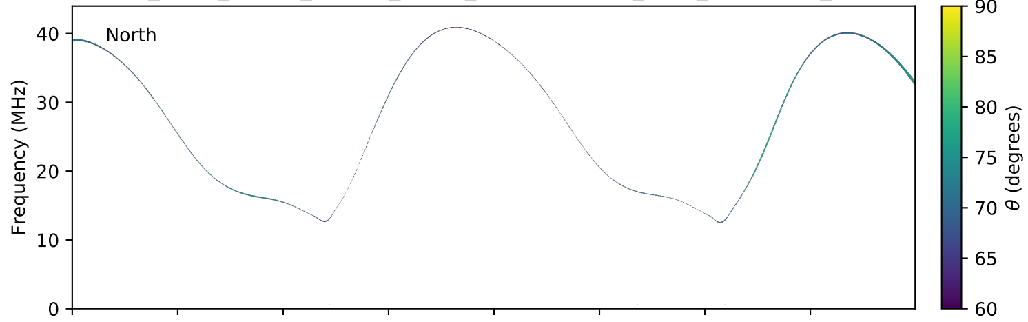
expres_earth_jupiter_europa_jrm09_lossc-wid1deg_3kev_20070103_v01.cdf
