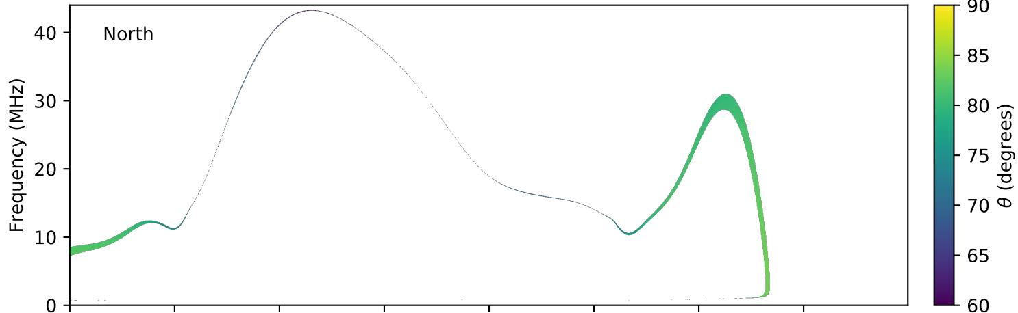
expres_earth_jupiter_io_jrm09_lossc-wid1deg_3kev_20061230_v01.cdf
