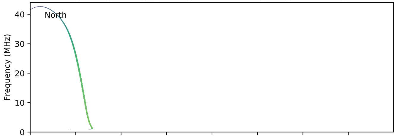
expres_earth_jupiter_io_jrm09_lossc-wid1deg_3kev_20061220_v01.cdf
