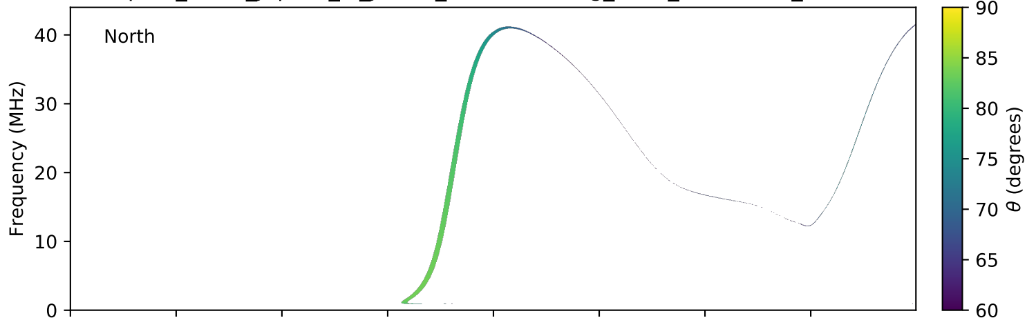
expres_earth_jupiter_io_jrm09_lossc-wid1deg_3kev_20061219_v01.cdf
