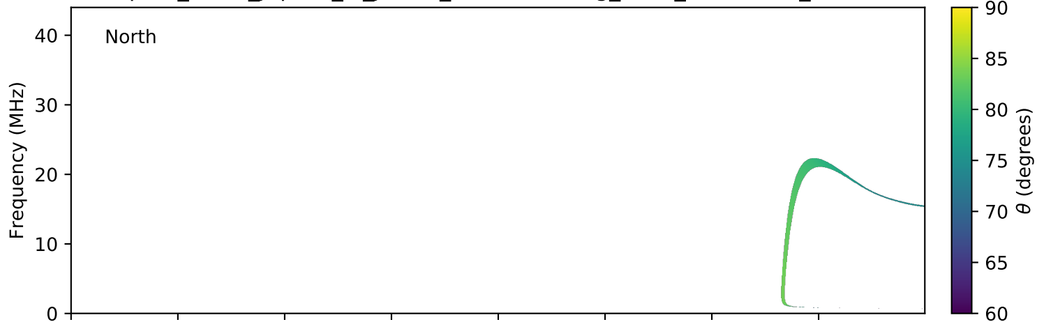
expres_earth_jupiter_io_jrm09_lossc-wid1deg_3kev_20061215_v01.cdf
